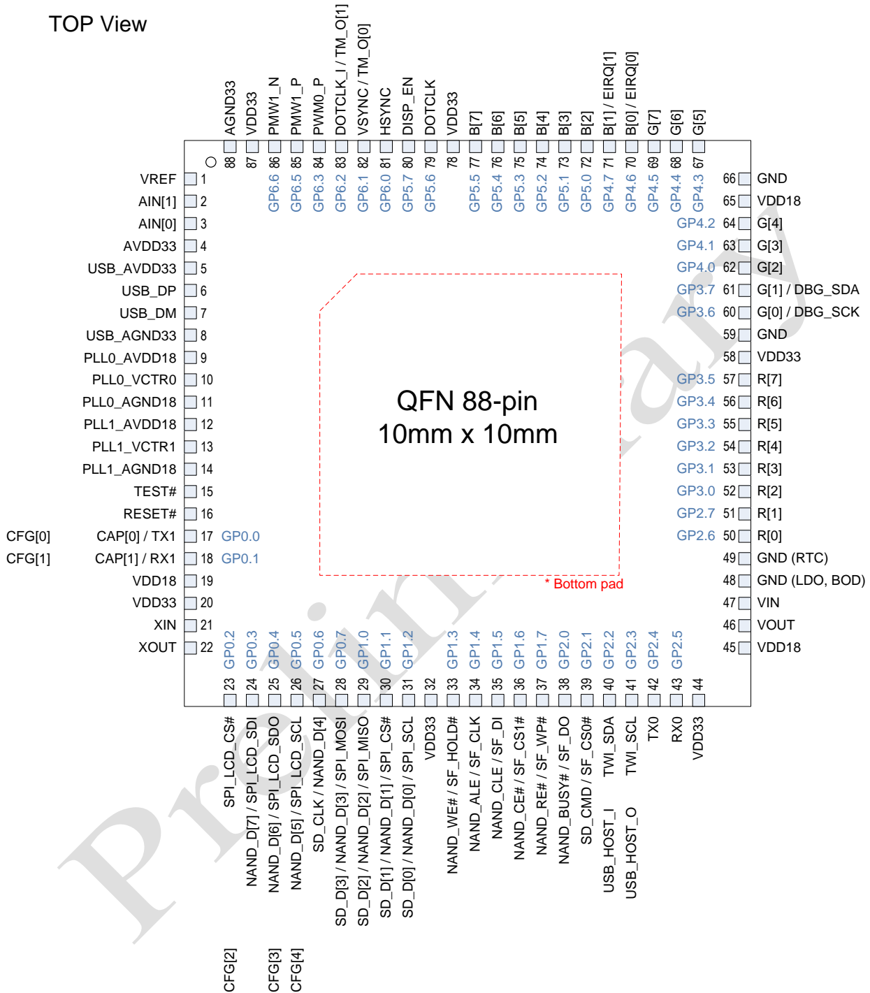
Figure 2-3 adStar-LxxN 88-Pin Layout
