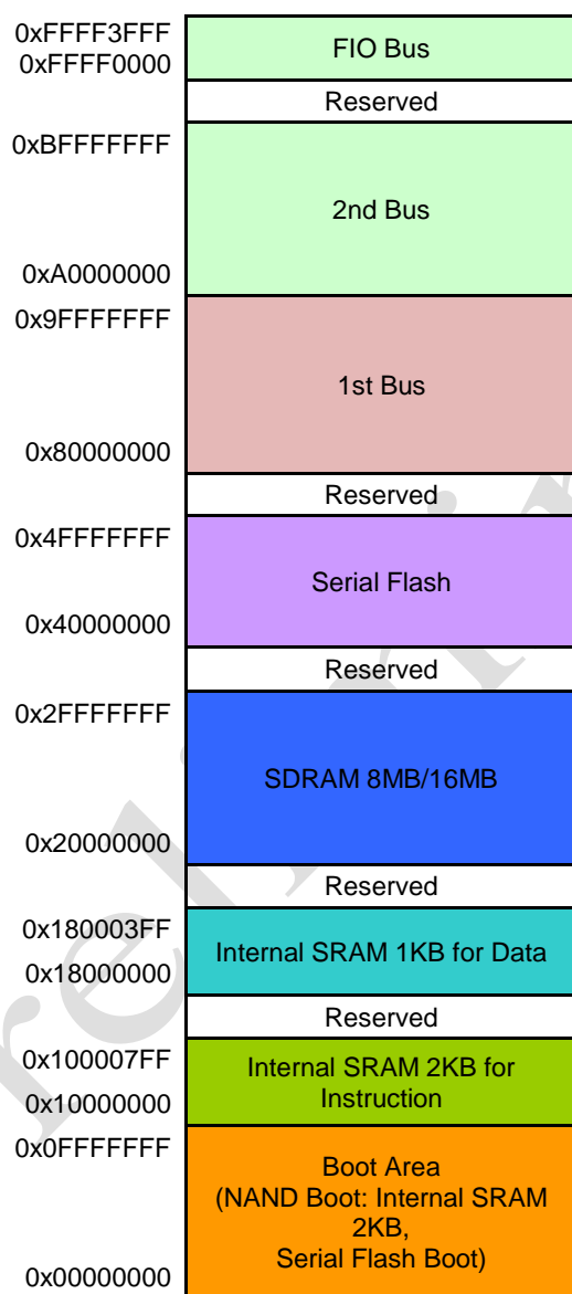
Figure 3-1 Memory Map
