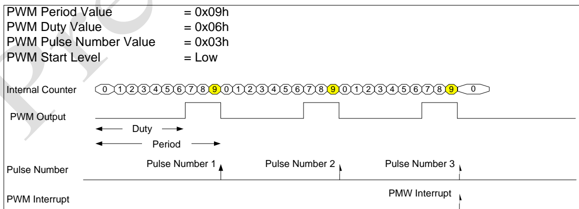
Figure 11-3 PWM Operation
