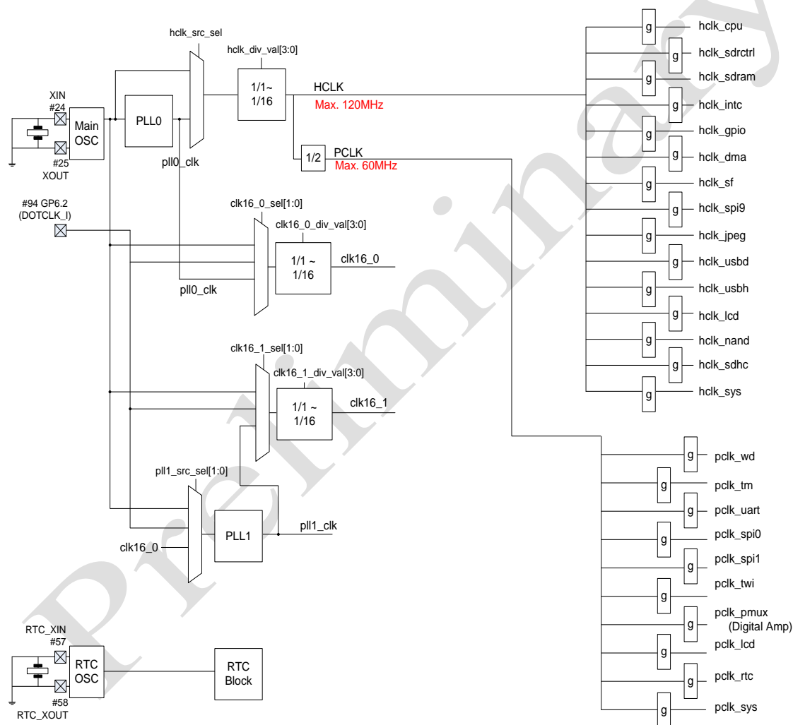
Figure 4-3 Clock Scheme
