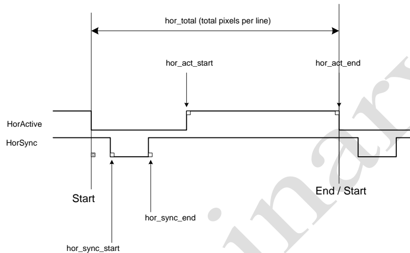
Figure 24-5 Horizontal Timing
